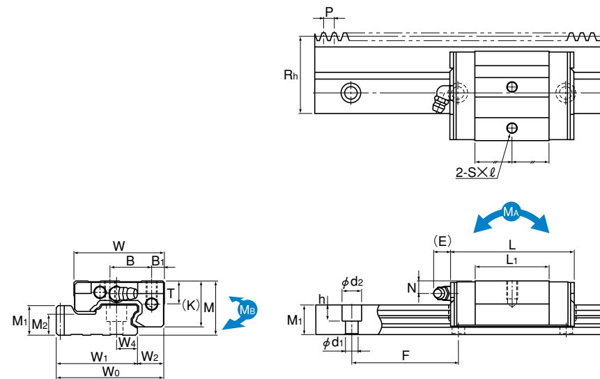
Model GSR25V-R
